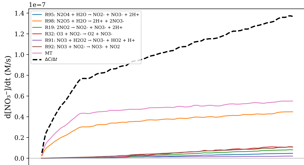
(a) \text{NO}_3^-
