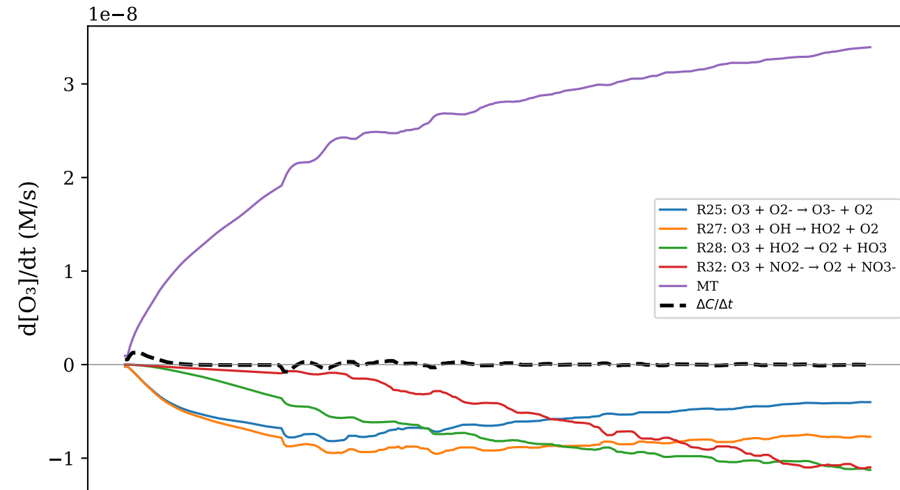
(b) \text{O}_3
